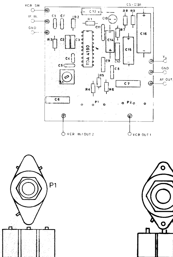
Figure 17 : PC Board and Components Layout of the Circuit of Fig. 16 (1 : 1 scale).
