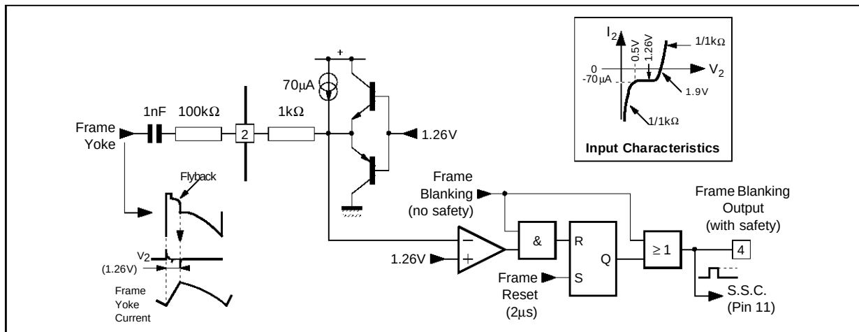
Figure 61 : Block Diagram
