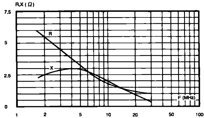
TYPICAL INPUT IMPEDANCE
