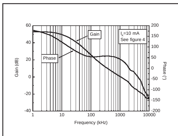
Gain &amp; Phase vs Frequency
