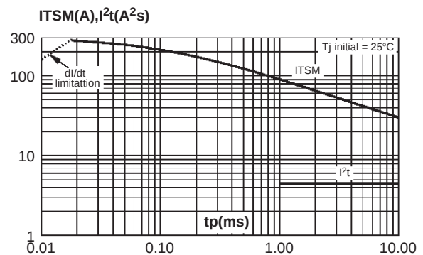
Fig. 9: Non-repetitive surge peak on-state current for a sinusoidal pulse with width t_p < 10\text{ ms} , and corresponding values of I t.
