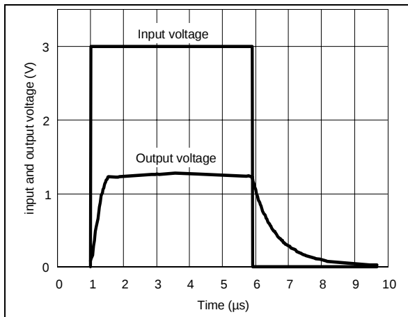
Pulse response at I_k = 1mA
