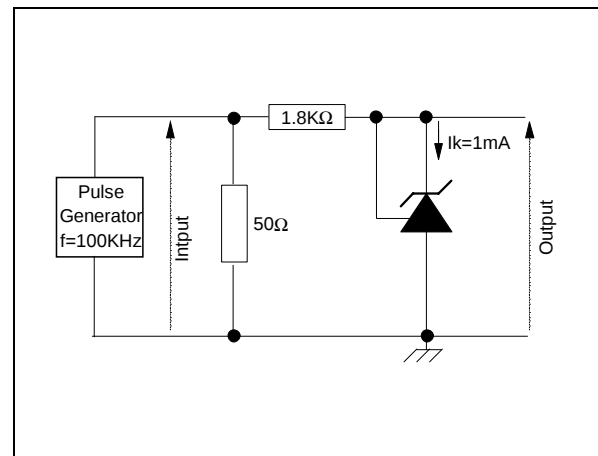
Test circuit for pulse response at I_k = 1mA
