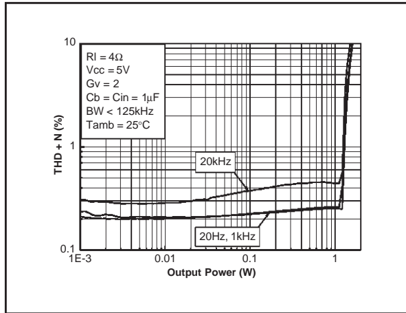
Fig. 27 : THD + N vs Output Power
