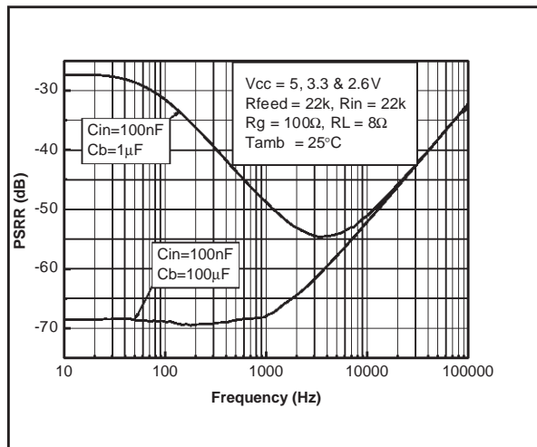
Fig. A : PSRR changes with Cb
