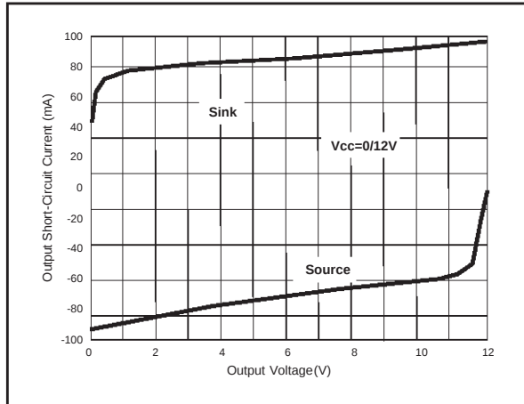
OUTPUT SHORT CIRCUIT CURRENT vs OUTPUT VOLTAGE
