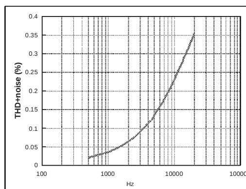
Figure 5 : THD+Noise versus Frequency (headphone outputs)
