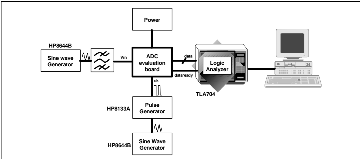
Figure 7 : Analog to Digital Converter characterization bench
