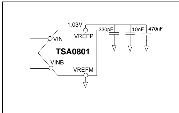
Figure 5 : Internal reference setting
