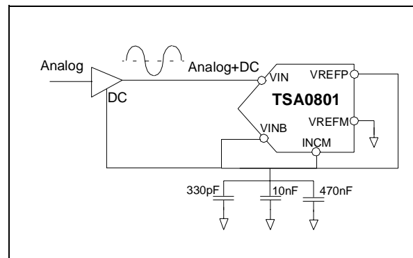
Figure 3 : DC-coupled 2Vpp analog input
