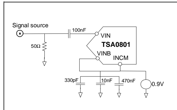
Figure2 : AC-coupled Single-ended input
