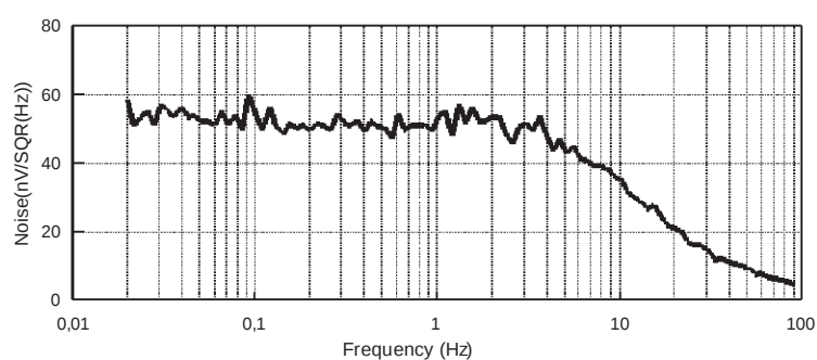
Noise = F(frequency)
