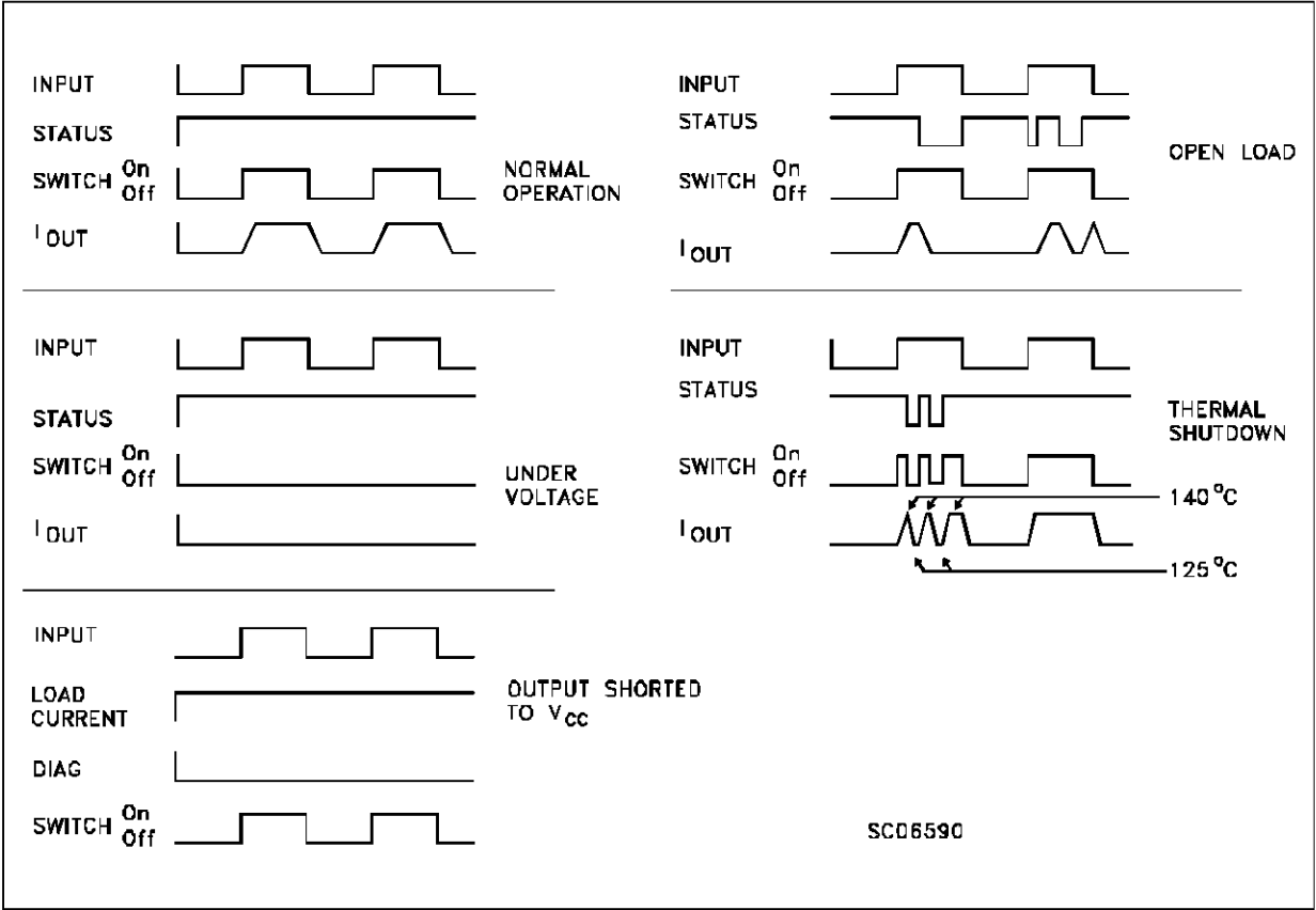
Figure 1: Waveforms
