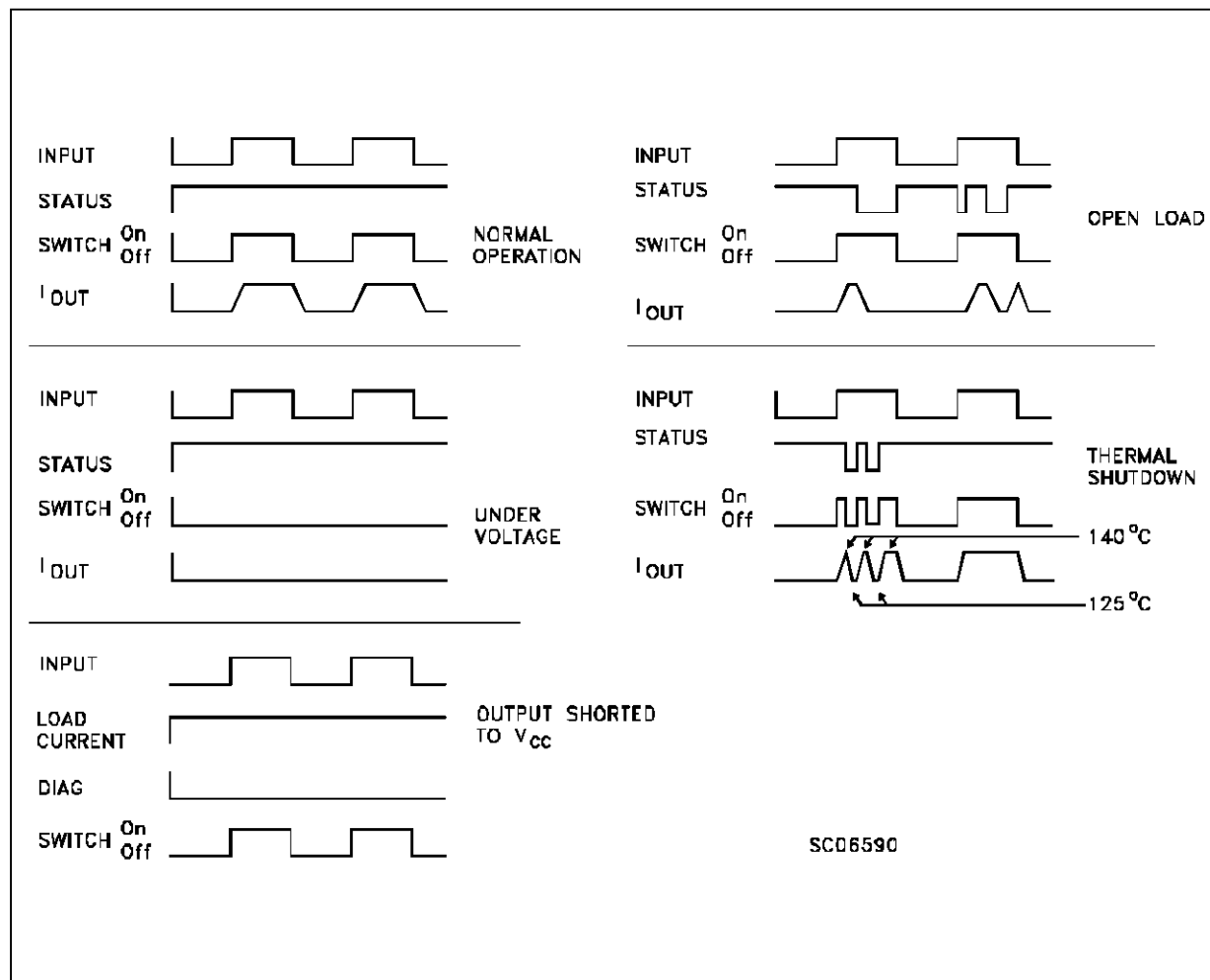
Figure 1: Waveforms
