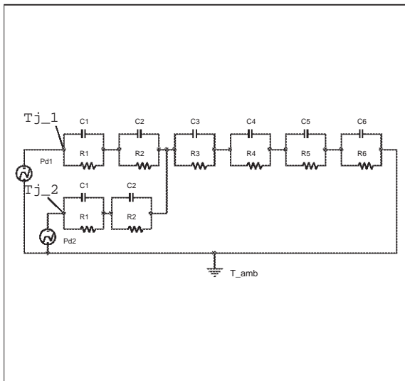
Thermal fitting model of a double channel HSD in PowerSO-10
