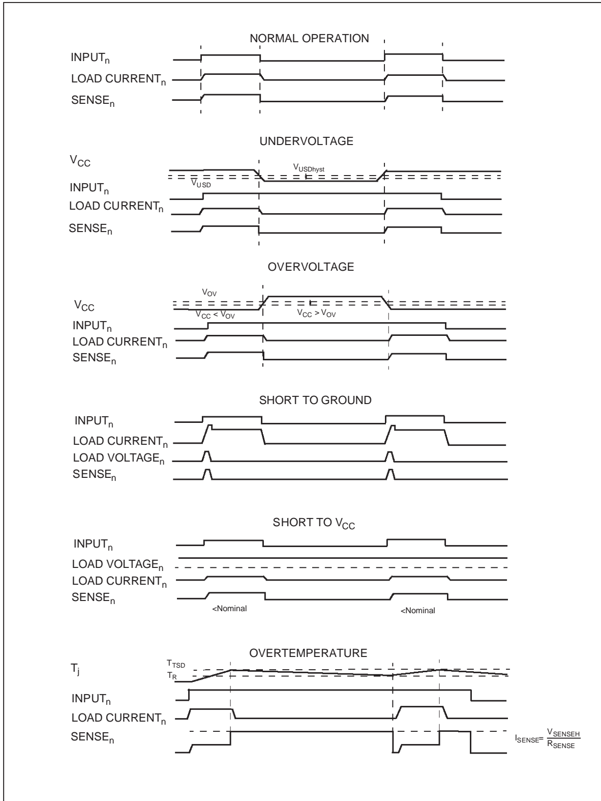
Figure 2: Waveforms
