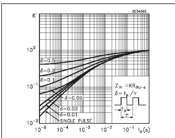
Thermal Impedance for DPAK/IPAK
