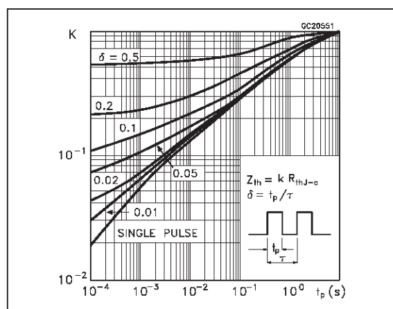
Thermal Impedance for SOT-223
