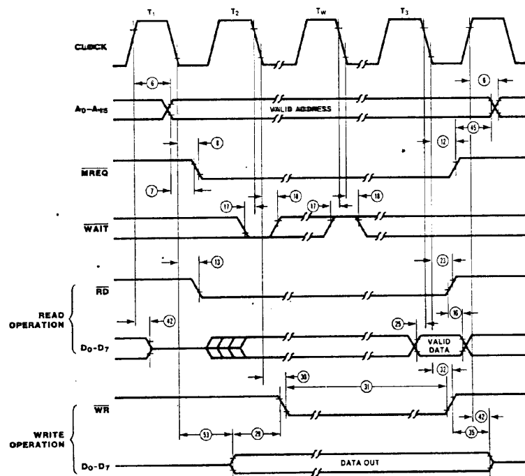
Figure 6. Memory Read or Write Cycles
