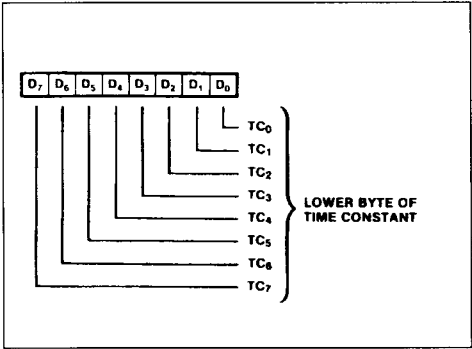
Figure 55 : Write Register 12.
