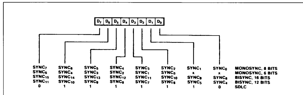
Figure 49 : Write Register 6.
