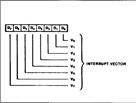
Figure 61 : Write Register 2.
