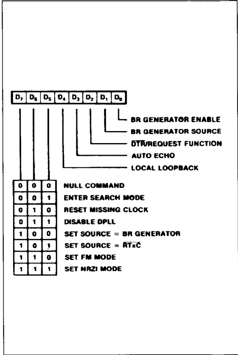
Figure 57 : Write Register 14.
