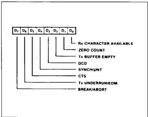
Figure 59 : Read Register 0.
