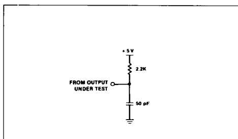
Figure 74 : Open-Drain Test Load.
