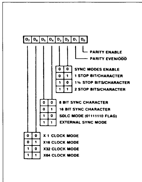
Figure 47 : Write Register 4.
