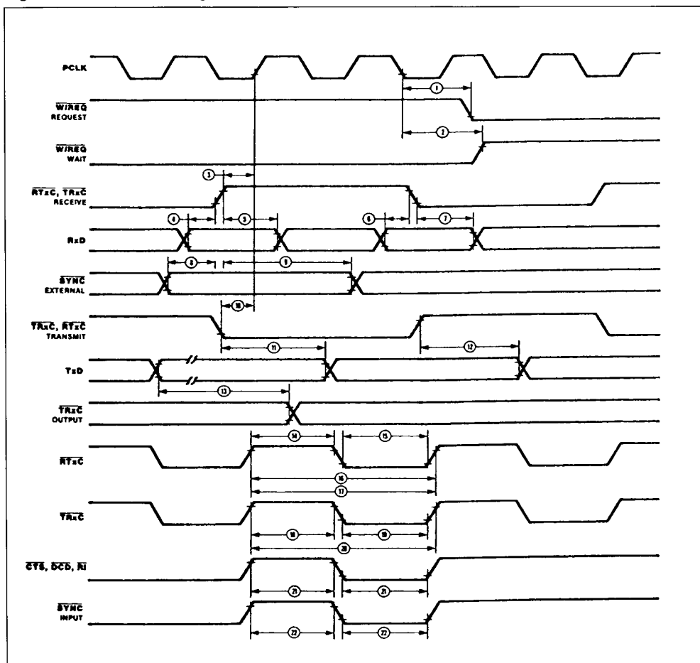
Figure 79 : General Timing.
