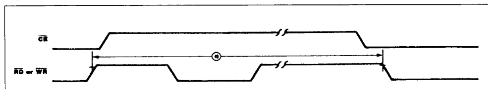
Figure 78 : Cycle Timing.
