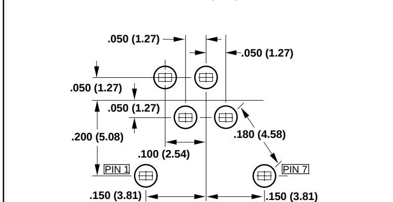
Y07C MOUNTING HOLE PATTERN
