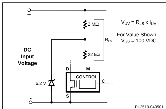
Figure 32. Line Sensing for Under-Voltage Only (Overvoltage Disabled).
