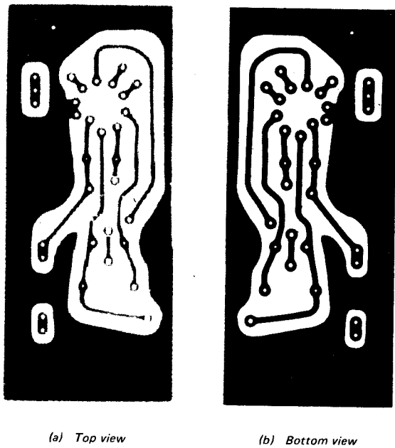
Fig. 9 – Printed circuit board for test circuit, full size (for TO-5 style package).
