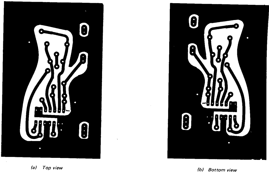
Fig. 11 – Printed circuit board for test circuit, full size (for 14-lead dual-in-line plastic package).
