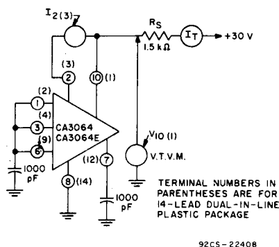
Fig.4 — Test setup: Measurement of total device dissipation, zener regulating voltage, quiescent operating current at terminal 2 (3).
