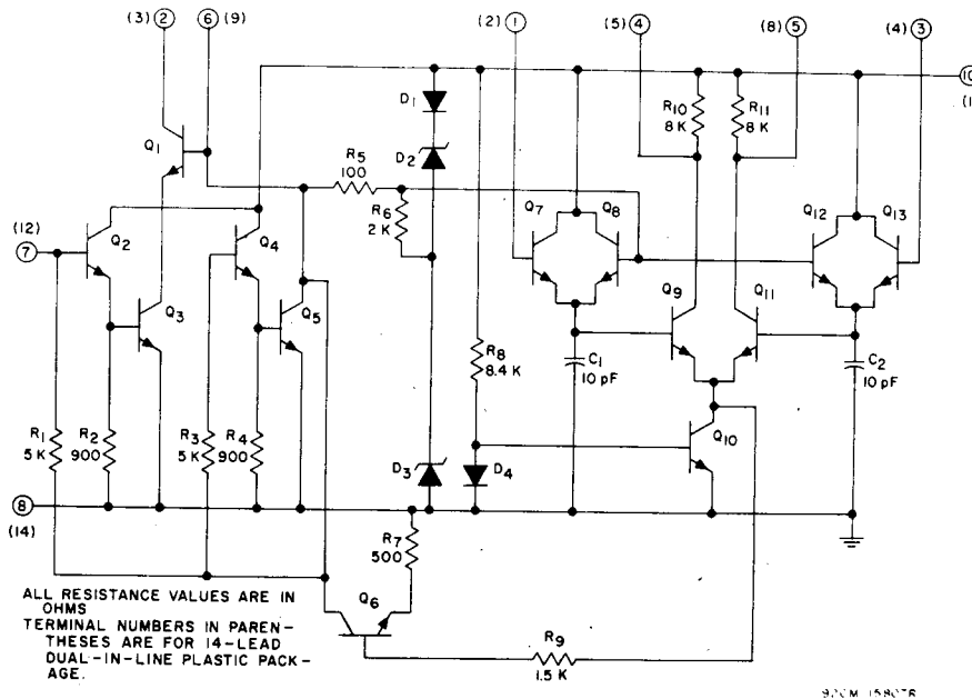
Fig.3 — Schematic diagram for CA3064 and CA3064E.
