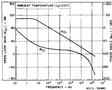
Fig. 11 — Open-loop gain and phase-shift response for CA3493.
