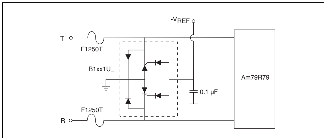
Figure 3.27 SLIC Protection with a Dual Battrax Device
