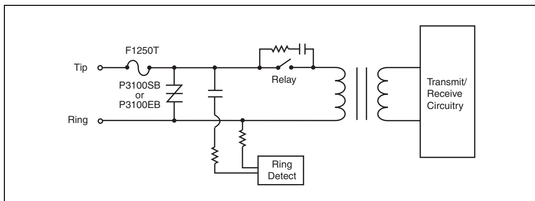
Figure 3.3 Modem Interface
