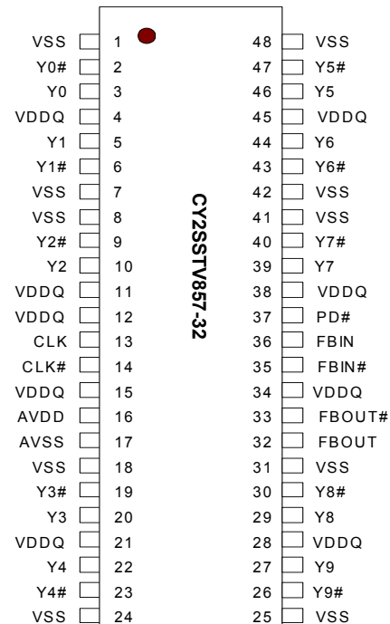
48 TSSOP Package
