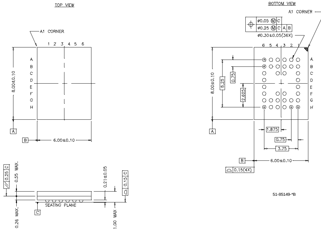
36-Lead FBGA (6 × 8 × 1 mm) BV36A
