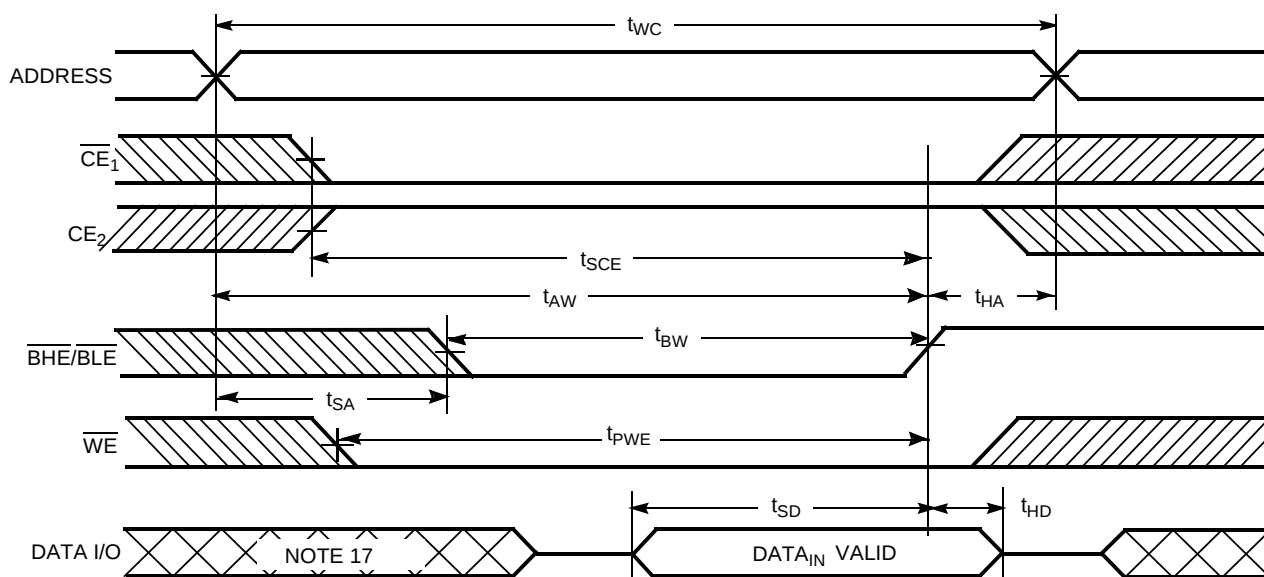
Write Cycle No. 4 ( \overline{\text{BHE/BLER}} Controlled, \overline{\text{OE}} LOW) [16]
