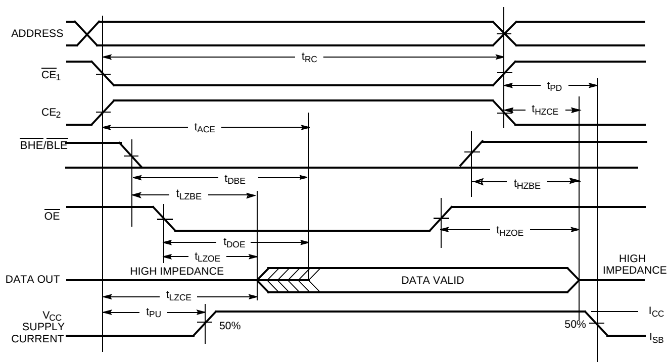
Read Cycle No. 2 ( \overline{OE} controlled) [13, 14]
