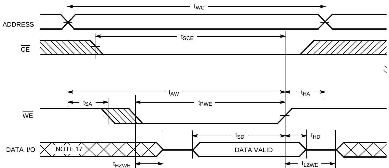
Write Cycle No. 2 (WE Controlled, OE LOW) [16]
