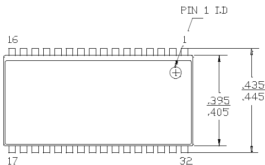
32-Lead (400-Mil) Molded SOJ V33
