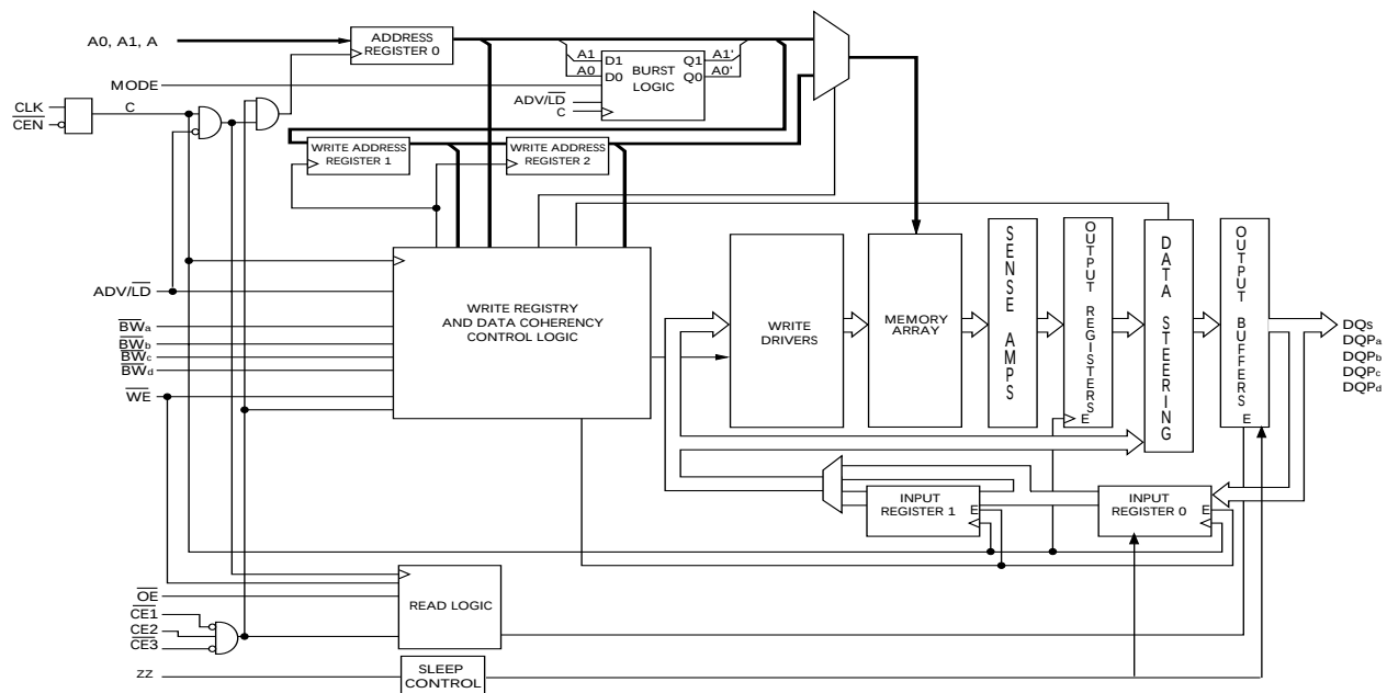
Logic Block Diagram-CY7C1354BV25 (256K x 36)
