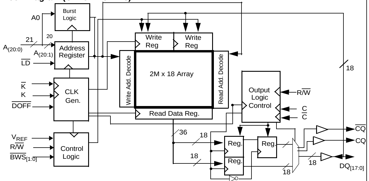
Logic Block Diagram (CY7C1418AV18)
