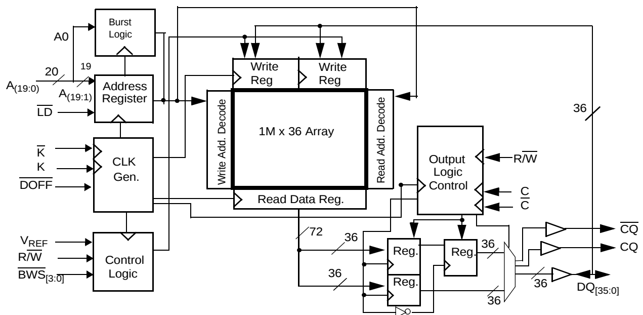
Logic Block Diagram (CY7C1420AV18)
