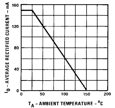
FIGURE 5 AVERAGE RECTIFIED CURRENT VS. AMBIENT TEMPERATURE
