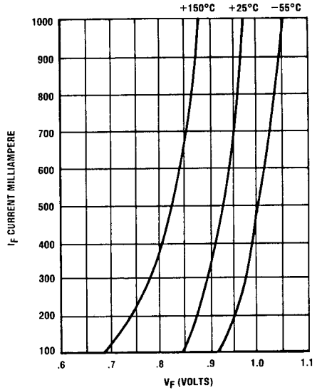
+150°C +25°C -55°C FIGURE 3 TYPICAL FORWARD CONDUCTANCE CURVE
