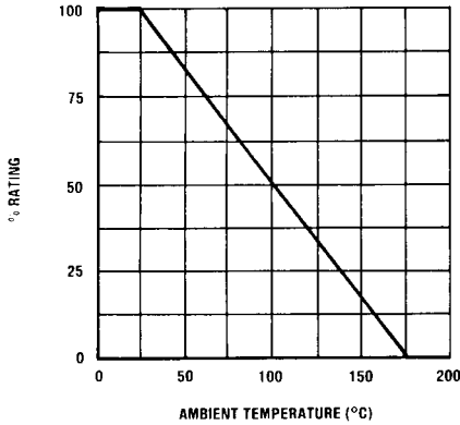
AMBIENT TEMPERATURE (°C) FIGURE 2 TEMPERATURE DERATING CURVE
