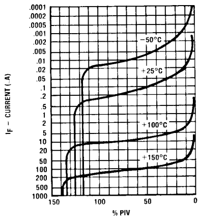
FIGURE 2 TYPICAL REVERSE CURRENT vs. PIV
