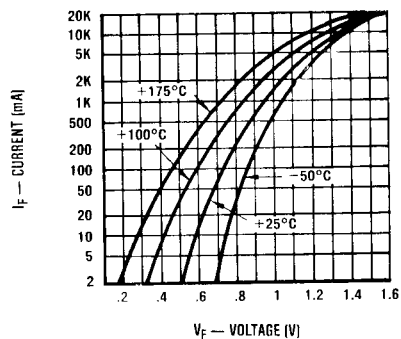
FIGURE 3 TYPICAL FORWARD CURRENT vs. FORWARD VOLTAGE
