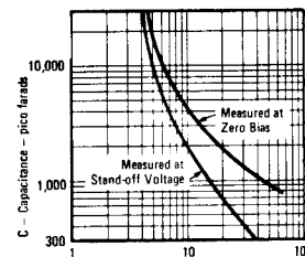
FIGURE 4 TYPICAL CAPACITANCE VS BREAKDOWN VOLTAGE (BIDIRECTIONAL TYPES)
