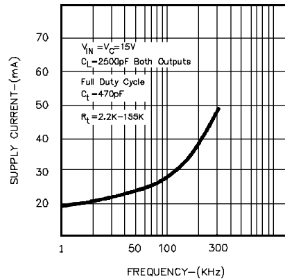
FIGURE 14. SUPPLY CURRENT VS. OUTPUT FREQUENCY
