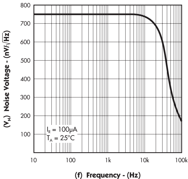
FIGURE 7. — NOISE VOLTAGE
