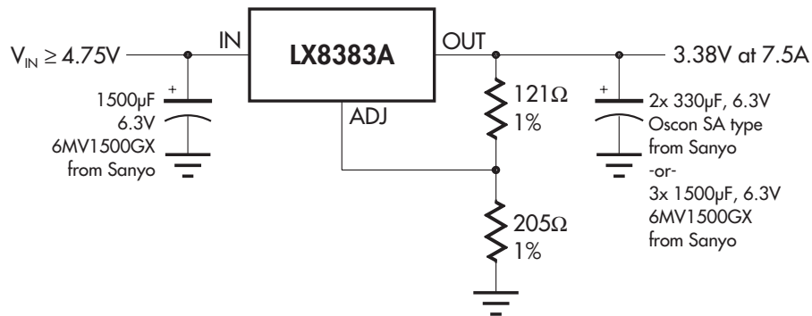
3.3V, 7.5A REGULATOR
