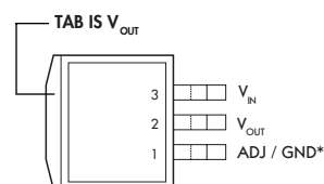
DD PACKAGE (Top View)
