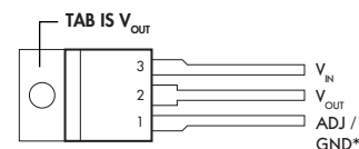
P PACKAGE (Top View)
