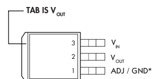
DD PACKAGE (Top View)
