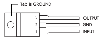
P PACKAGE (Top View)
