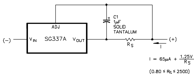
FIGURE 10 - CURRENT REGULATOR
