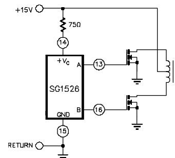
FIGURE 25. DRIVING N-CHANNEL POWER MOSFETS
