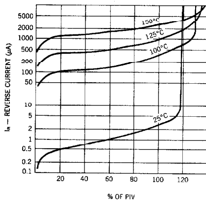
Typical Reverse Current vs Voltage
