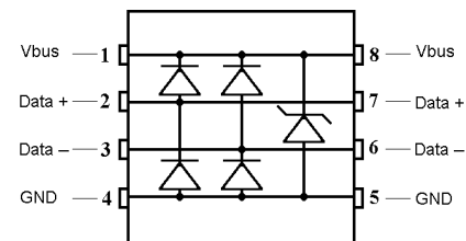
SCHEMATIC
