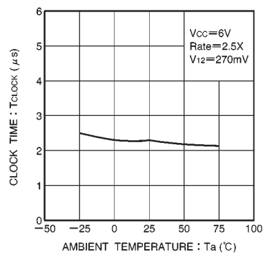
Fig. 13 Clock period vs. ambient temperature (I)
