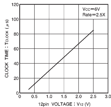
Fig. 16 Clock period vs. pin 12 voltage
