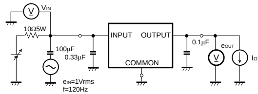
Fig. 2 Measurement circuit for ripple rejection ratio
