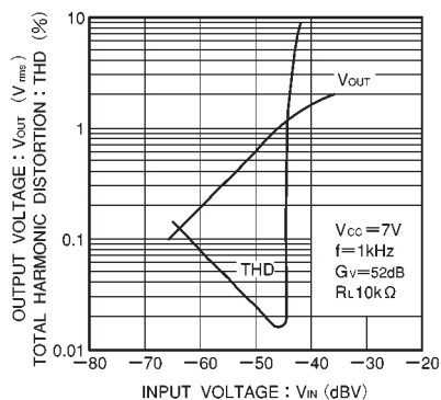
Fig. 18 Input/output characteristics
