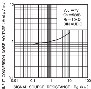
Fig. 15 Input conversion noise voltage vs. signal source resistance
