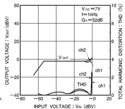
Fig. 17 ALC characteristics
