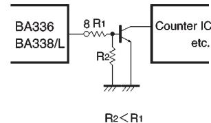
Fig. 5 Circuit example
