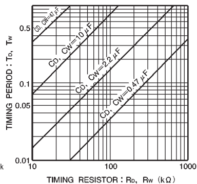
Fig. 8 Relation of external capacitors and resistors to mute detection time T_D and output pulse width T_W
