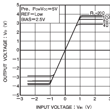
Fig.5 Driver I / O characteristics (When \text{Pre } V_{CC} = \text{Pow } V_{CC} , with load regulation)
