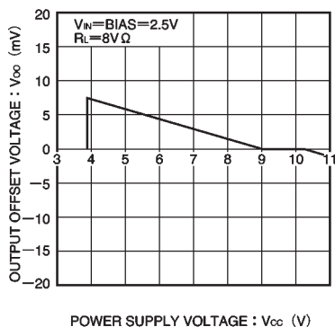
Fig.7 Power supply voltage vs. output offset voltage
