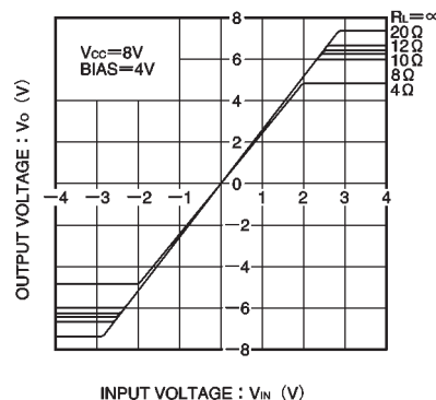
Fig.6 Driver I/O characteristics (VCC=8V)
