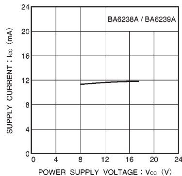
Fig.10 Supply current vs. power supply voltage
